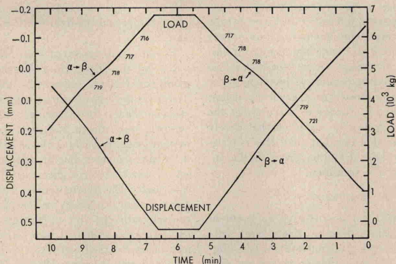
Fig. 5a. Tracing of load-displacement record for the 29th ( \beta \rightarrow \alpha ) and 30th ( \alpha \rightarrow \beta ) passage through the transition of run 602 (Table 2) at 3-kb confining pressure. Numbers along the load trace are sample temperatures in degrees C. The load pen led the displacement pen by the equivalent of 7-8 sec. The transition is marked by softening of the sample and can usually be seen in both the load and the displacement curves.
