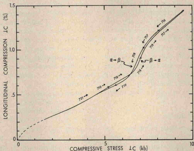
Fig. 5b. Stress-strain curve constructed from record of Figure 5a shows more clearly the softening that marks the transition as well as the hysteresis. The straightish section in the \beta field does not extrapolate to the origin because about 1-kb stress is needed to seat the various surfaces in the load column before the value 7 \times 10^{-6} cm/kg taken for apparatus distortion is valid. The lack of coincidence below the transition stress of the curves of increasing and decreasing stress is unusually large in this example, and we have no ready explanation for it.
